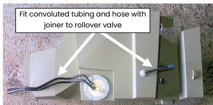
Photo 2: Tank preparation
