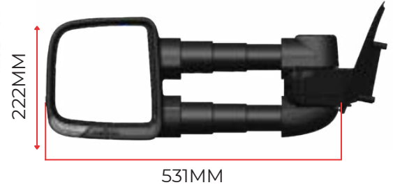
Fully Extended Towing Position
